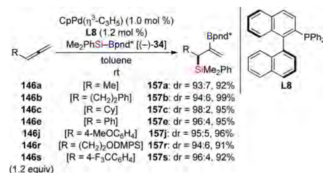
Scheme 57. Reagent- and Catalyst-Controlled Diastereoselective Silaboration of Allenes
