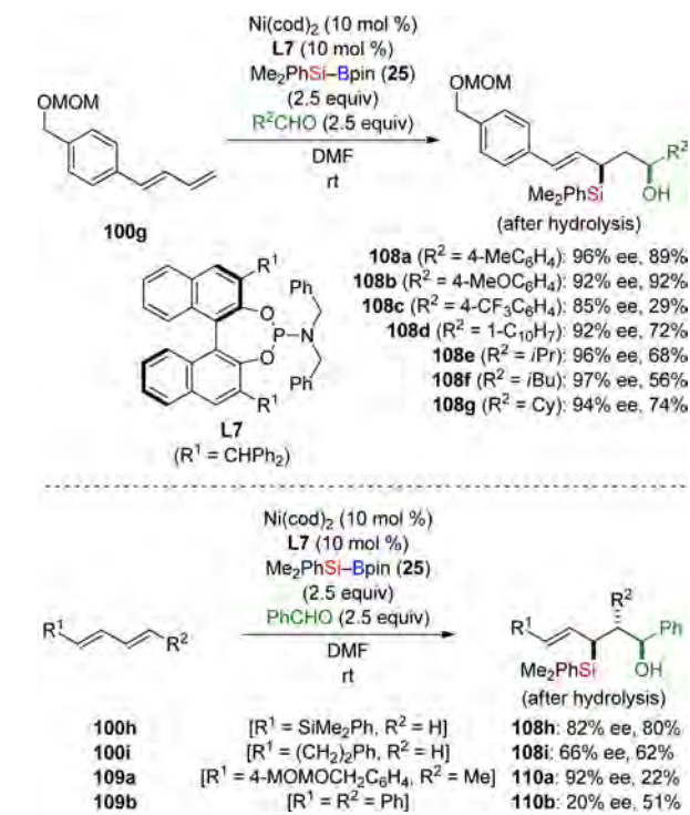
Scheme 42. Nickel(0)-Catalyzed Three-Component Coupling of 1,3-Dienes, Aldehydes, and \text{Me}_2\text{PhSi-Bpin} (25)
