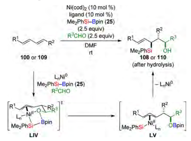
Scheme 41. Plausible Pathway of the Nickel(0)-Catalyzed Three-Component Reaction
