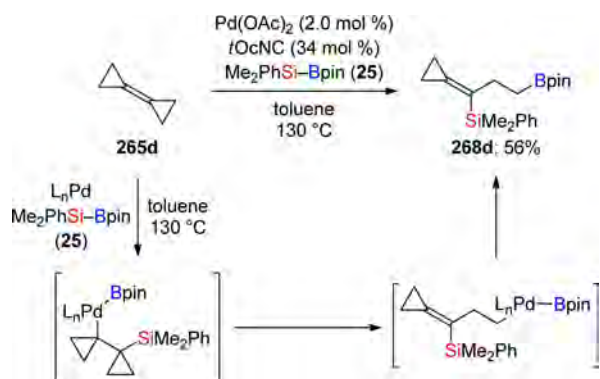
Scheme 92. Addition of Me 2 PhSi–Bpin (25) to Bicyclopolyidene (265d)
