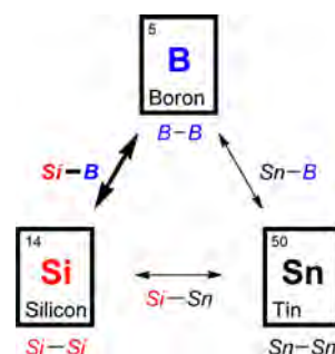
Figure 1. Interelement compounds from boron, silicon, and tin.
