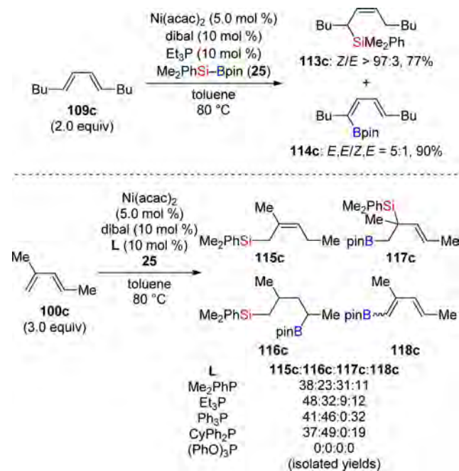
Scheme 44. Disproportionation in the Silaboration of Acyclic Buta-1,3-dienes with Terminal Substitution
