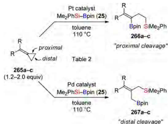
Scheme 90. Selective Distal or Proximal C–C Bond Cleavage
