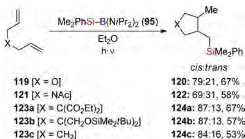
Scheme 46. Silylative Radical 5- Exo -Cyclization of 1,6-Dienes
