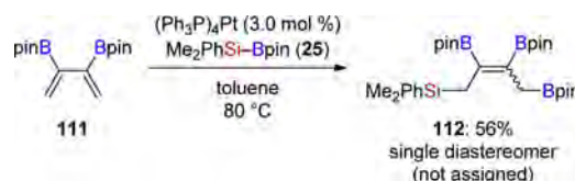
Scheme 43. Silaboration of Diborated Buta-1,3-diene 111
