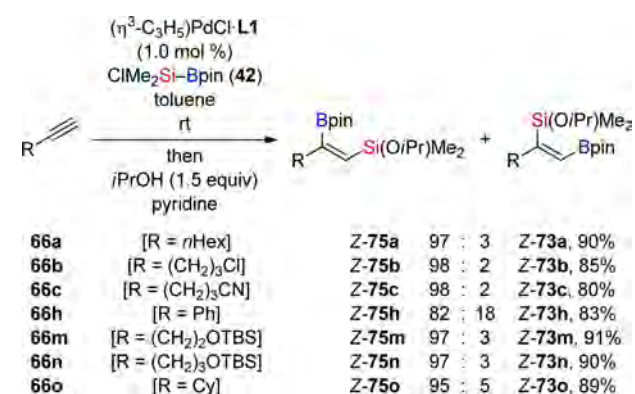
Scheme 19. Inverse Regioselectivity in the Silaboration of Terminal Alkynes
