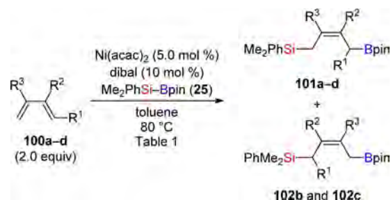
Scheme 36. 1,4-Silaboration of Acyclic 1,3-Dienes
