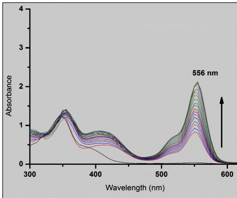
Fig. 1. UV-vis absorption spectra of probe L in presence of \text{Cu}^{2+} solution.
