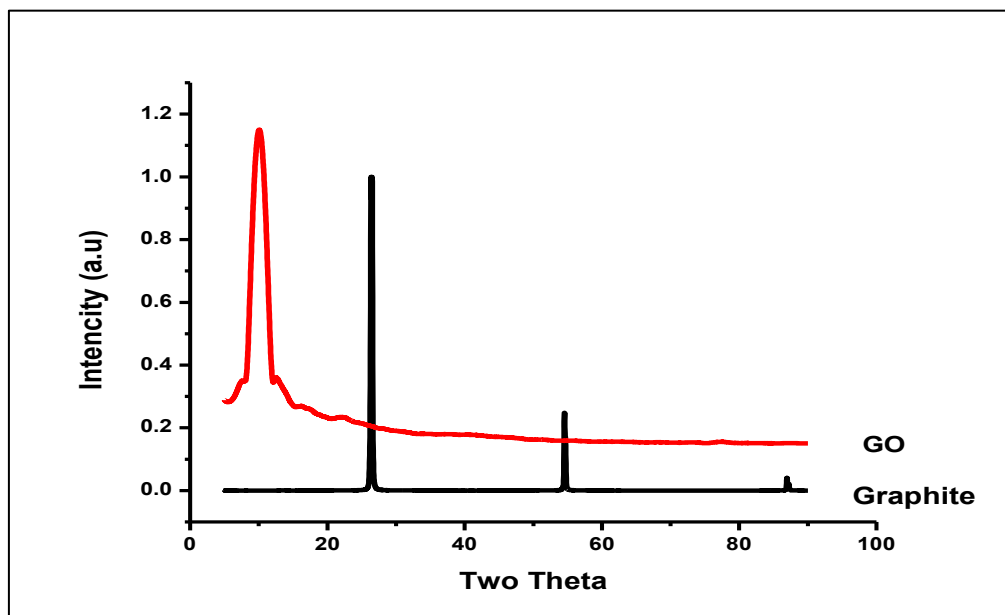
Fig.-5: XRD OF G.O. & GRAPHITE.
