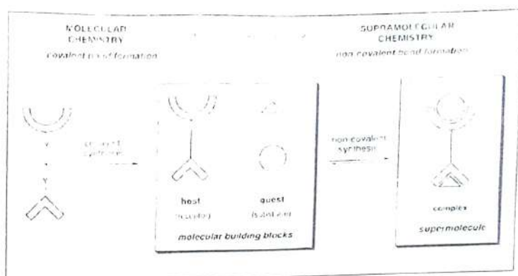
Figure 1. From molecular to supramolecular chemistry: molecules, supermolecules.
