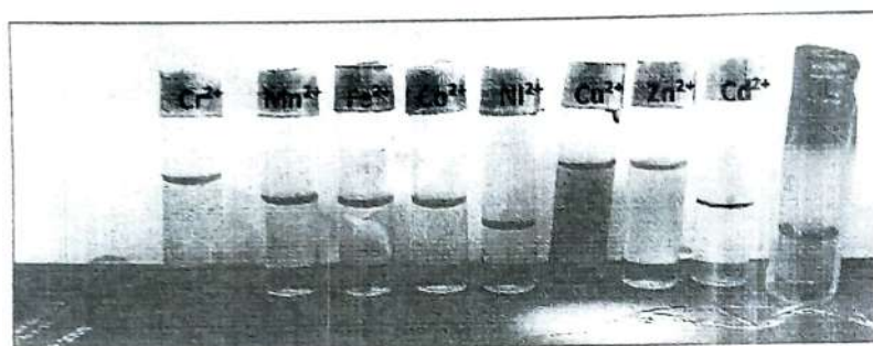
Visible colour change of chemosensor in presence of various metal ions
