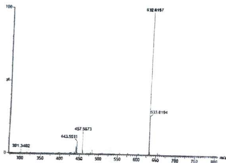
Mass spectrum of probe L
