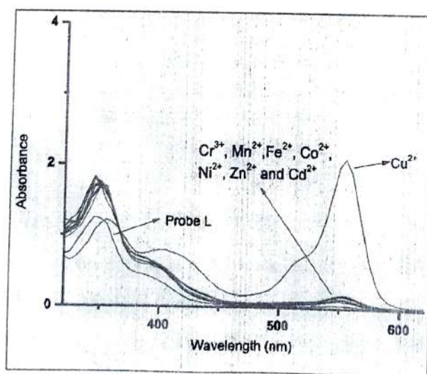
Fig.2. UV-vis absorption spectra of probe L in presence of various cations.
