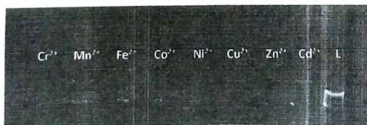
Fluorescent colour change of chemosensor- L in presence of various metal ions
