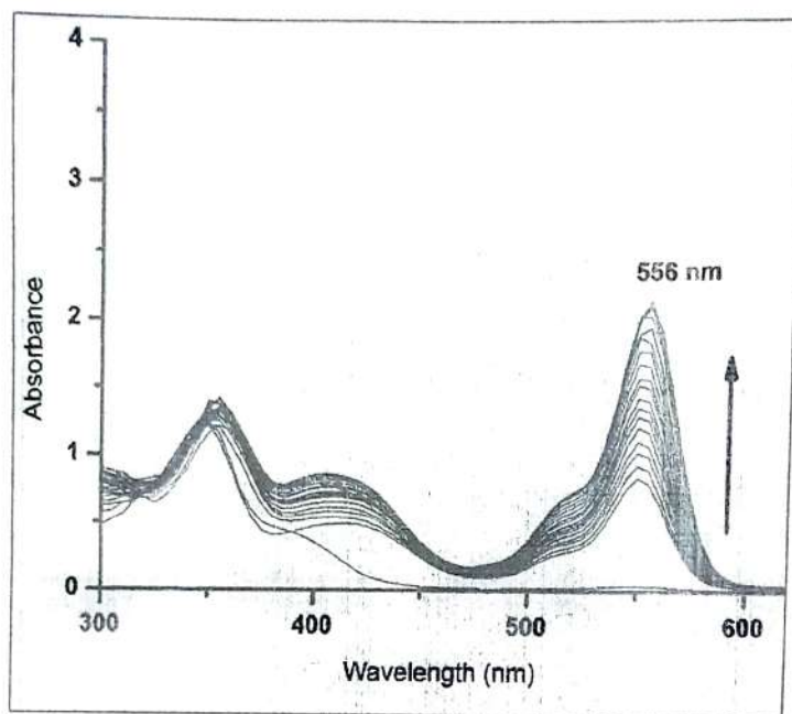
Fig. 1. UV-vis absorption spectra of probe L in presence of \text{Cu}^{2+} solution.
