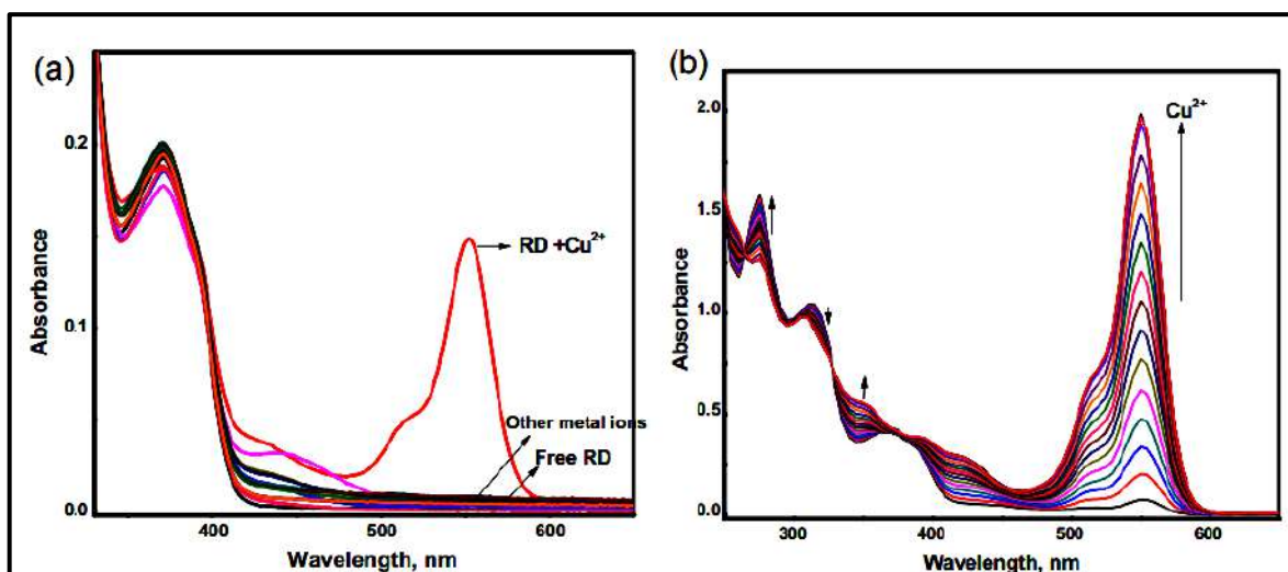
(a) UV-vis spectra of RD ( 10 \mu\text{M} ) with metal ions in \text{CH}_3\text{CN}/\text{H}_2\text{O} (7:3 v/v) solution. (b) UV-vis spectra of RD ( 10 \mu\text{M} ) with \text{Cu}^{2+} (0– 20 \mu\text{M} ) in \text{CH}_3\text{CN}/\text{H}_2\text{O} (7:3 v/v) solution.
